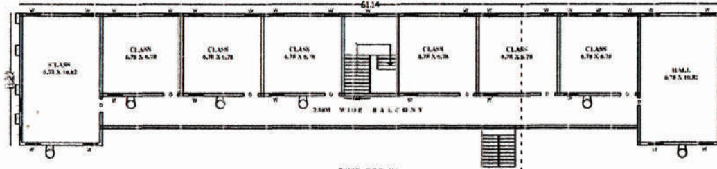
EXIST. S.F. PLAN
